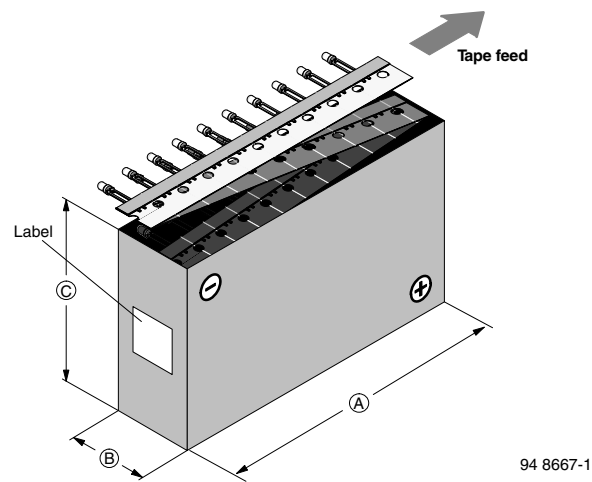
Fig. 19 - Tape Direction
