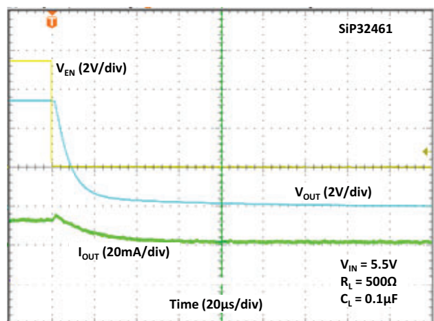
Fig. 43 - Turn-off Time
