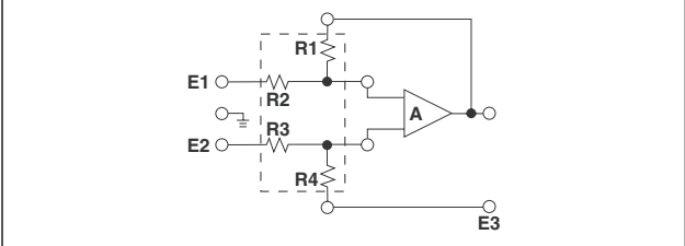
Figure 4—Model 300198 Network (application example)
