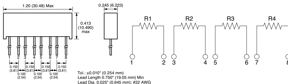
Figure 7 – Molded 2R, 3R, 4R Resistor Network Dimensions and Circuit Design in inches (millimeters)
