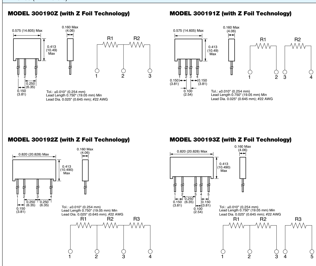
Figure 5—Molded 2R, 3R, 4R Resistor Network Dimensions and Circuit Design in inches (millimeters)
