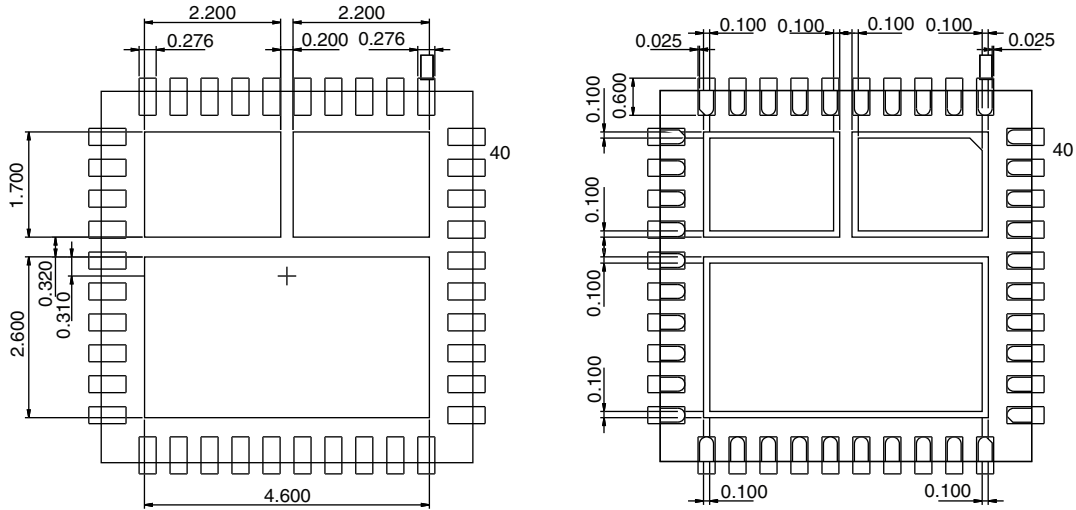
Figure 8 - PowerPAK MLP 66-40
