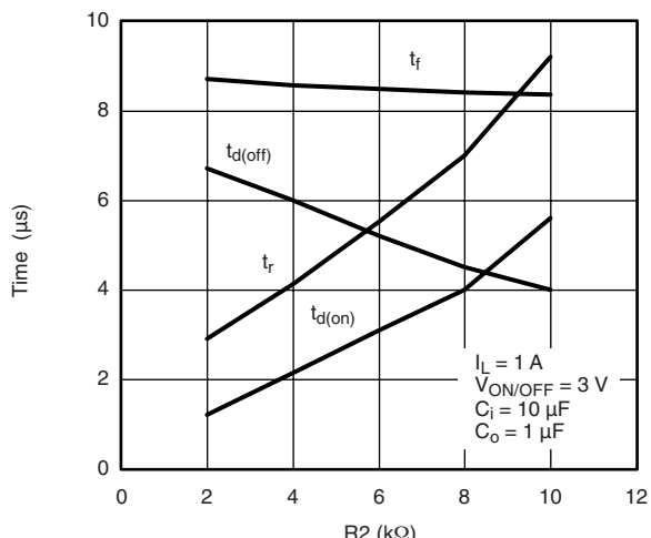
Switching Variation R2 at V_IN = 5 V, R1 = 20 kΩ
