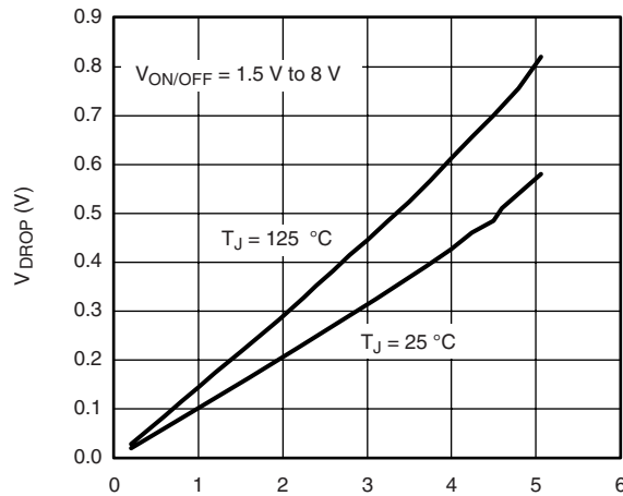
V DROP vs. I L at V IN = 5 V
