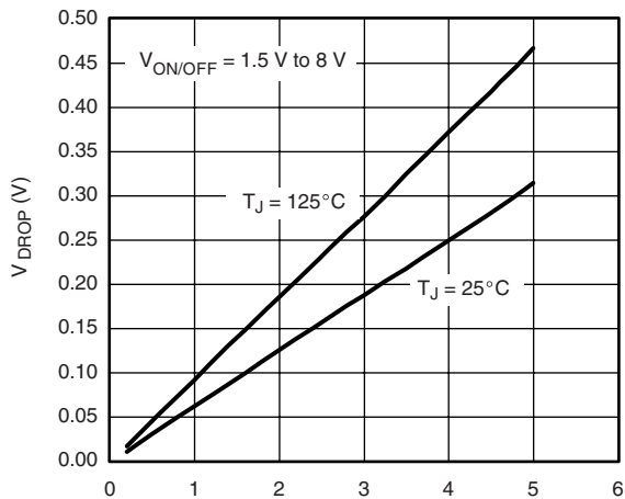
V DROP vs. I L at V IN = 10 V
