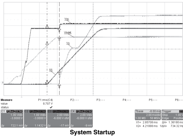
System Startup
