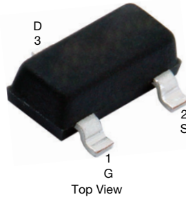
SC-70 (3 leads) SOT-323
