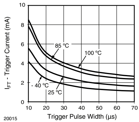
20015 Fig. 10 - I_{FT} vs. LED Pulse Width
