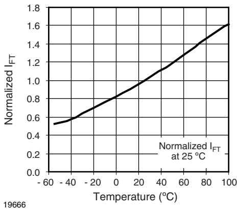
19666 Fig. 7 - Normalized Trigger Input Current vs. Temperature
