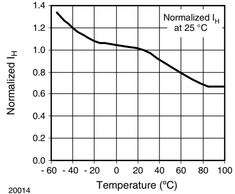
20014 Fig. 9 - Normalized I_H vs. Temperature
