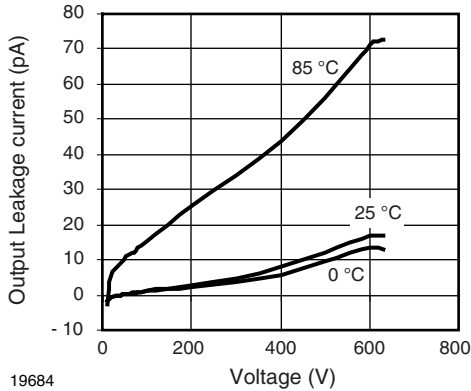
19684 Fig. 6 - Output Off Current (Leakage) vs. Voltage
