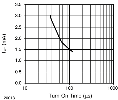
20013 Fig. 8 - I_{FT} vs. Turn-On Time ( \mu s )
