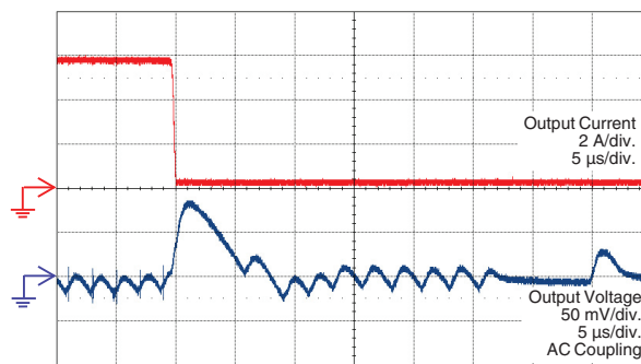
Transient Response in Power Save Mode (6 A to 0.2 A) (V IN = 12 V, V OUT = 1 V, f sw = 500 kHz at 6 A)
