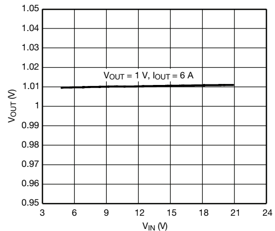
V_{OUT} vs. V_{IN} at I_{OUT} = 6\text{ A} (in Continuous Conduction Mode, f_{SW} = 500\text{ kHz} )
