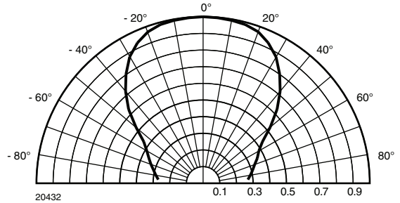
Fig. 12 - Directivity
