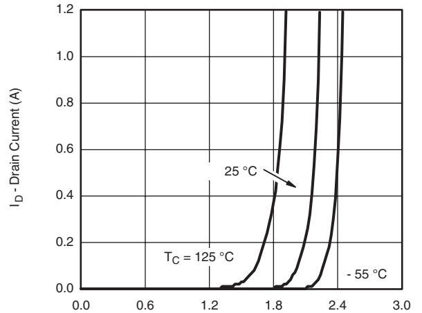
T_C = 125 \text{ °C} and -55 \text{ °C} Transfer Characteristics
