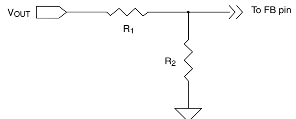
Fig. 3 - Output Voltage Selection
