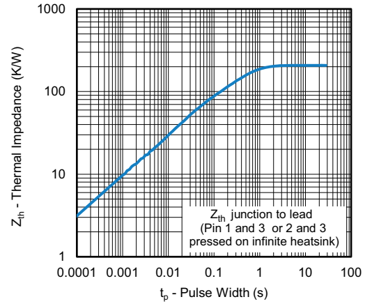
Fig. 10 - Thermal Impedance vs. Time
