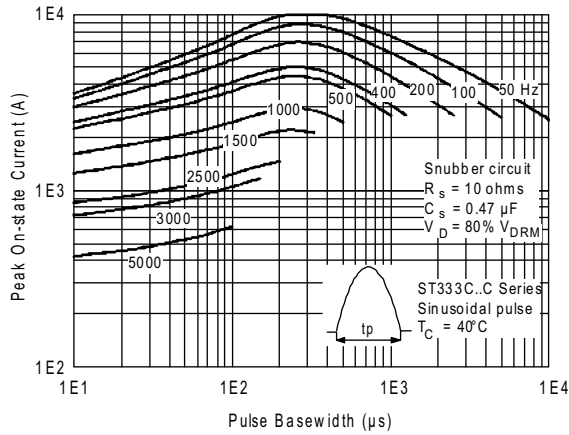
Fig. 13 - Frequency Characteristics
