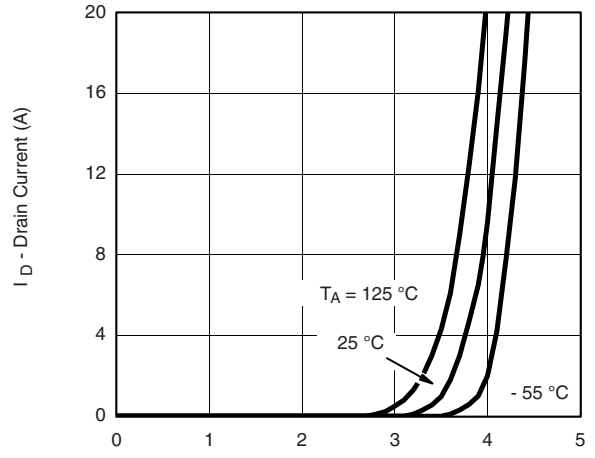
T_A = 125\text{ }^\circ\text{C} 25 °C -55 °C Transfer Characteristics
