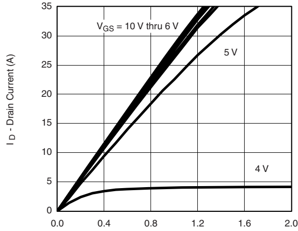
V_{GS} = 10 V thru 6 V Output Characteristics
