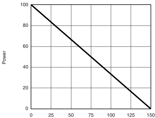
Power, Junction-to-Case
