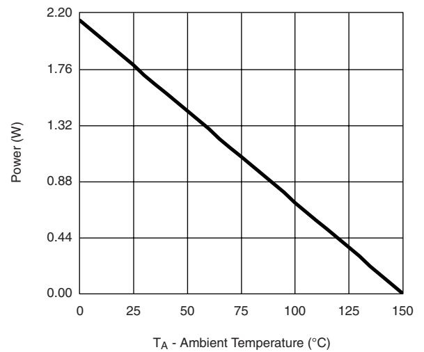
Power, Junction-to-Ambient
