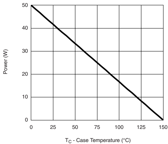
Power, Junction-to-Case
