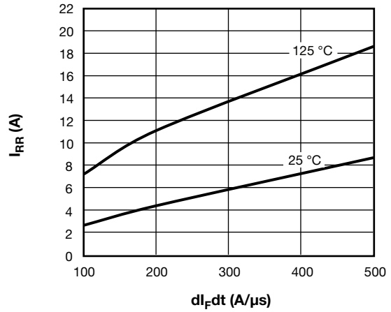
Fig. 15 - Typical D5 - D6 Clamping Diode Reverse Recovery Current vs. dI_F/dt , V_{rr} = 200 V, I_F = 50 A
