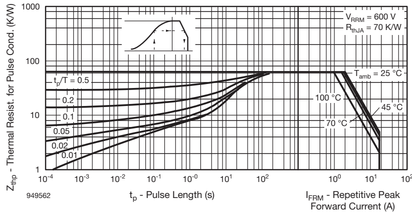
Fig. 8 - Thermal Response
