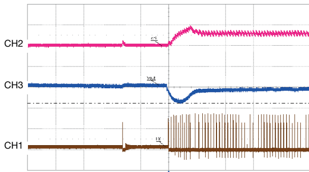
Fig. 11 - Load Step Undershoot Response, I_{OUT} = 0 \text{ A} to 3 \text{ A} CH2 (RED) = I_{COIL} (5 A/div), CH3 (BLU) = V_{OUT} (200 mV/div), CH1 (BRN) = LX (10 V/div), Time = 10 \mu\text{s}/\text{div}
