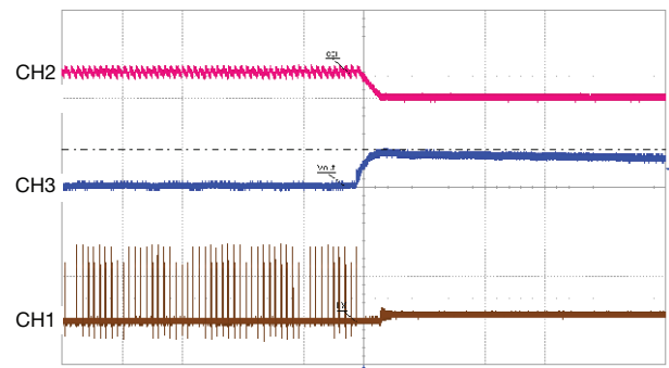
Fig. 14 - Load Step Overshoot Response, I_{OUT} = 3 \text{ A} to 0 \text{ A} CH2 (RED) = I_{COIL} (5 A/div), CH3 (BLU) = V_{OUT} (200 mV/div), CH1 (BRN) = LX (10 V/div), Time = 10 \mu\text{s}/\text{div}
