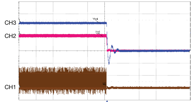
Fig. 18 - Shut-Down, I_{OUT} = 6\text{ A} CH1 (BRN) = LX (10 V/div), CH3 (BLU) = V_{OUT} (0.5 V/div), CH2 (RED) = I_{COIL} (5 A/div), Time = 200 \mu\text{s} /div
