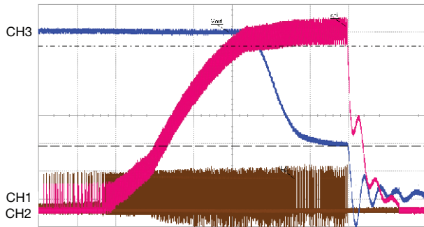
Fig. 17 - Over Current Protection, I_{VALLEY} = 6\text{ A} CH2 (RED) = I_{COIL} (1 A/div), CH3 (BLU) = V_{OUT} (200 mV/div), CH1 (BRN) = LX (10 V/div), Time = 100 \mu\text{s} /div
