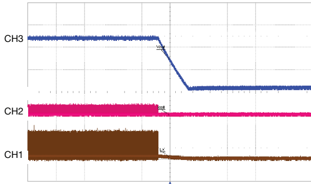
Fig. 16 - Shut-Down, I_{OUT} = 0\text{ A} CH1 (BRN) = LX (10 V/div), CH3 (BLU) = V_{OUT} (0.5 V/div), CH2 (RED) = I_{COIL} (2 V/div), Time = 5 ms/div
