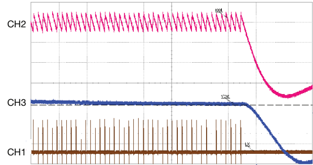
Fig. 19 - Over Current Protection, I_{VALLEY} = 6\text{ A} CH2 (RED) = I_{COIL} (1 A/div), CH3 (BLU) = V_{OUT} (200 mV/div), CH1 (BRN) = LX (10 V/div), Time = 10 \mu\text{s} /div
