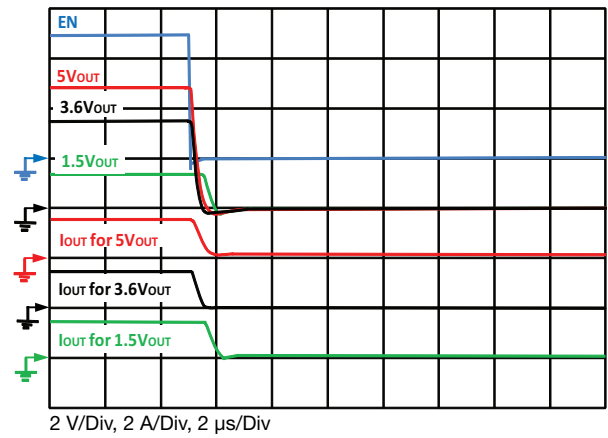
Fig. 22 - Typical Fall Time C_{OUT} = 0.1 \mu F, C_{IN} = 4.7 \mu F, I_{OUT} = 1.5 A
