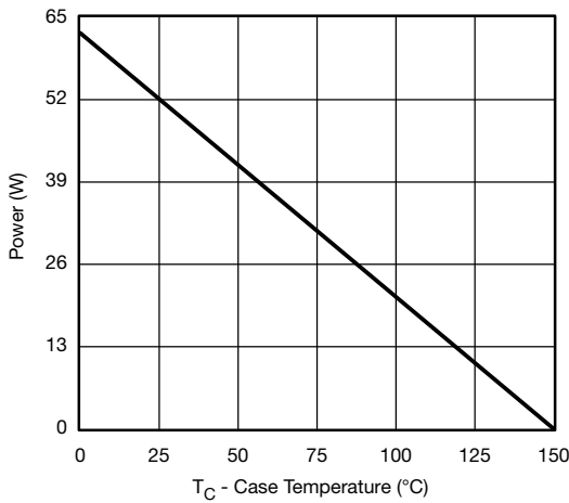
Power, Junction-to-Case
