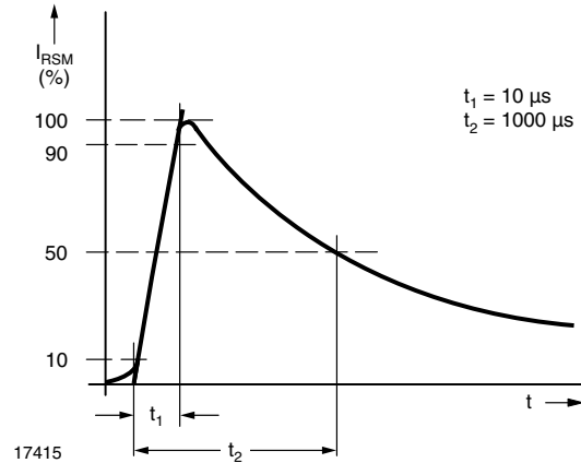
Fig. 4 - Pulse Waveform
