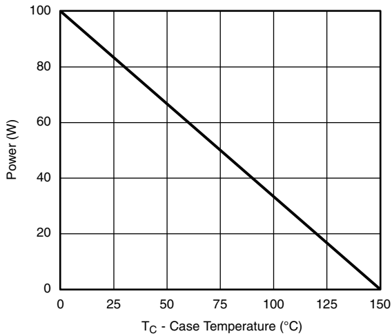
Power, Junction-to-Case
