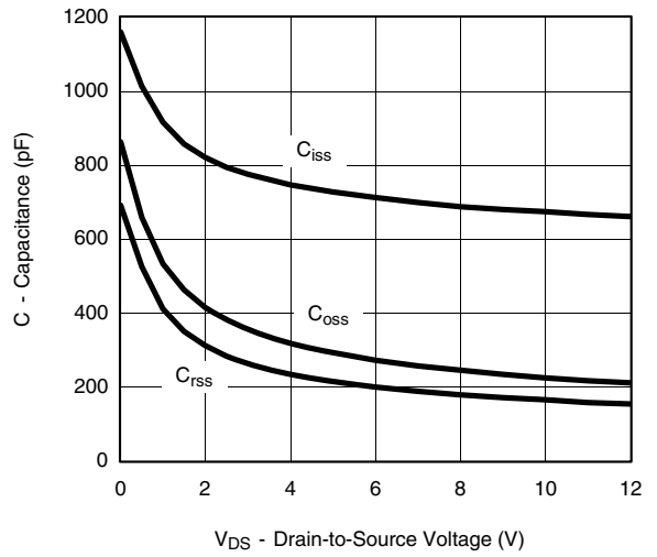
C - Capacitance (pF) V_{DS} - Drain-to-Source Voltage (V) Capacitance
