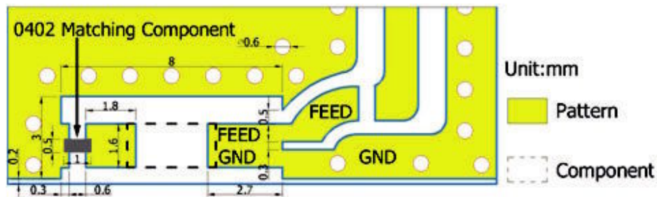
Land Pattern
