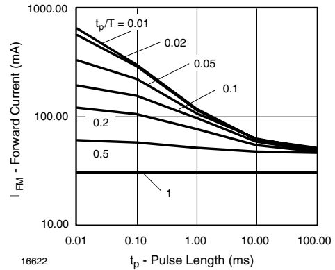
16622 t_p - Pulse Length (ms) Figure 10. Forward Current vs. Pulse Length
