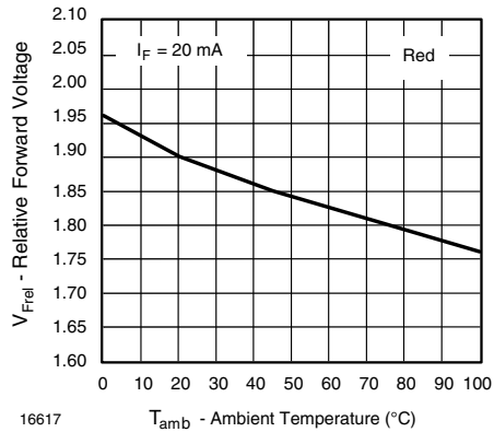
16617 T_{amb} - Ambient Temperature (°C) Figure 9. Forward Voltage vs. Ambient Temperature
