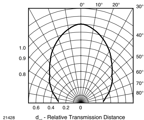
Fig. 11 - Vertical Directivity
