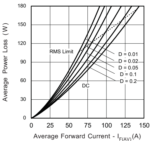
Fig. 5 - Forward Power Loss Characteristics (Per Leg)
