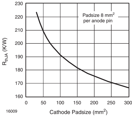
Fig. 5 - Thermal Resistance Junction Ambient vs. Cathode Padsize
