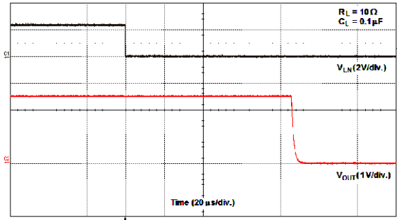
Fig. 28 - SiP32453 Turn-Off Time ( V_{IN} = 2.5 V )
