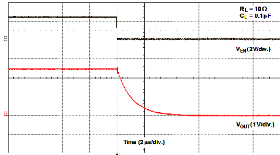
Fig. 27 - SiP32451 and SiP32452 Turn-Off Time ( V_{IN} = 2.5 V )
