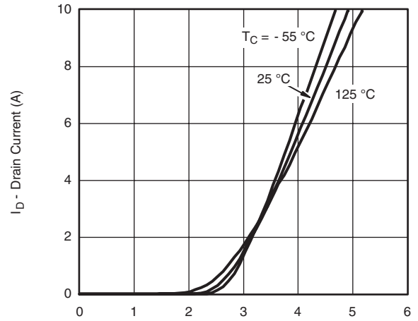
T_C = -55\text{ }^\circ\text{C} 25\text{ }^\circ\text{C} 125\text{ }^\circ\text{C} Transfer Characteristics
