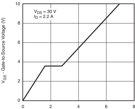
V_{DS} = 30\text{ V} I_D = 2.2\text{ A} Gate Charge
