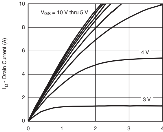
V_{GS} = 10\text{ V thru } 5\text{ V} Output Characteristics
