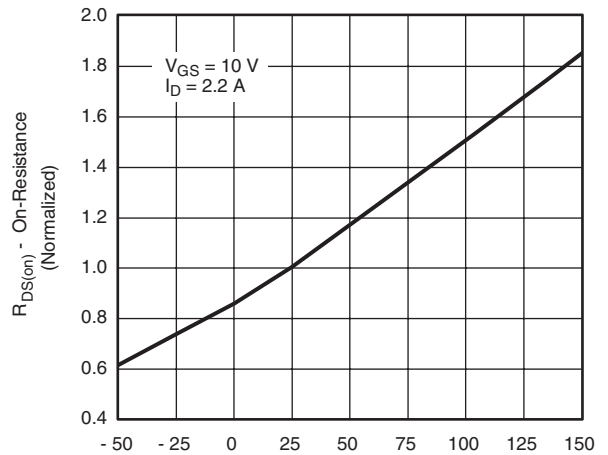
V_{GS} = 10\text{ V} I_D = 2.2\text{ A} On-Resistance vs. Junction Temperature
