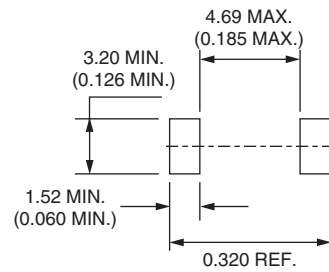
Soldering pad
