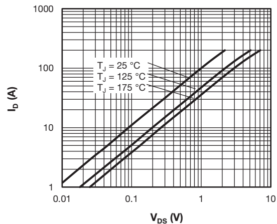
Fig. 2 - Typical MOSFET Output Characteristics, V GS = 10 V
