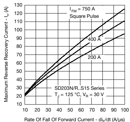
Fig. 15 - Recovery Current Characteristics
