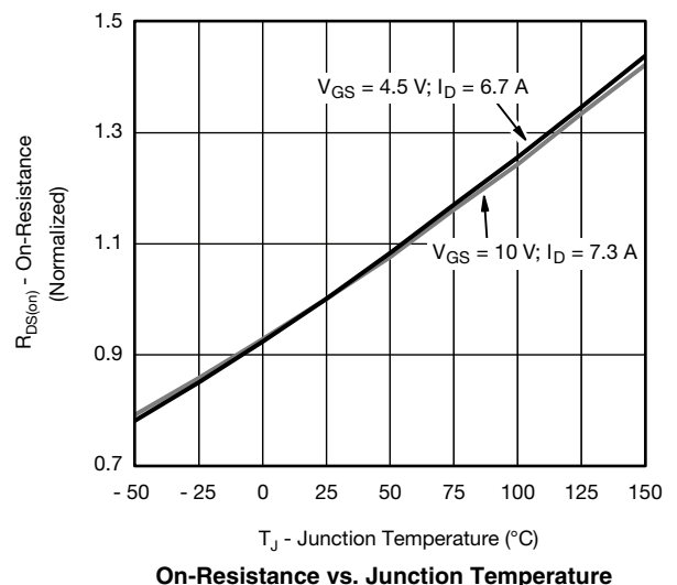
V_{GS} = 4.5\text{ V}; I_D = 6.7\text{ A} V_{GS} = 10\text{ V}; I_D = 7.3\text{ A} On-Resistance vs. Junction Temperature
