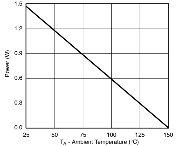
Power Derating
