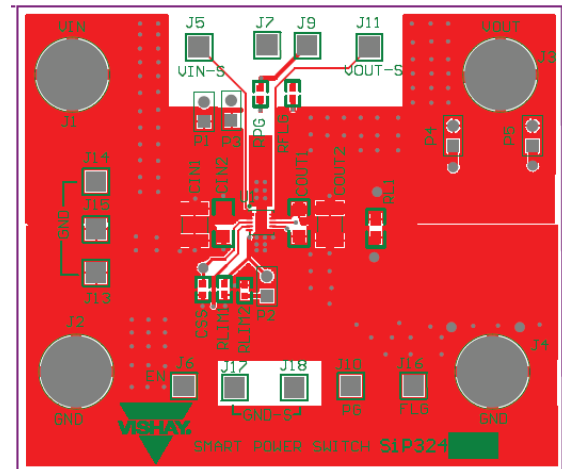
Fig. 49 - Application Board Layout
