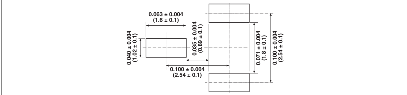
FIGURE 6 - RECOMMENDED LAND PATTERN
