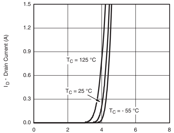
T_C = 125\text{ }^\circ\text{C} T_C = 25\text{ }^\circ\text{C} T_C = -55\text{ }^\circ\text{C} Transfer Characteristics
