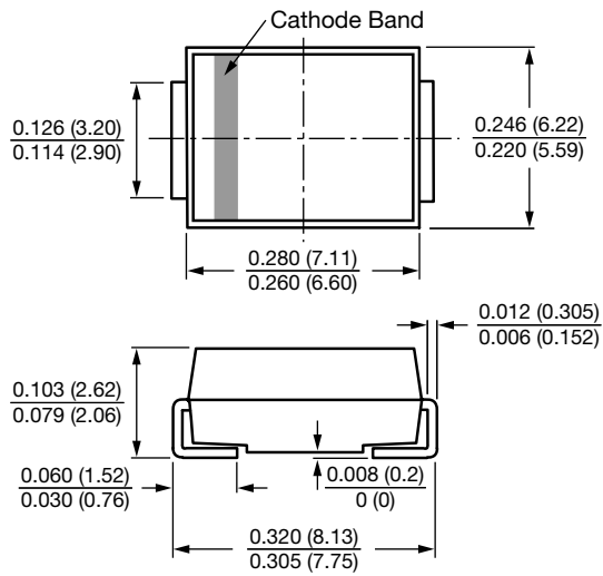
SMC (DO-214AB)
