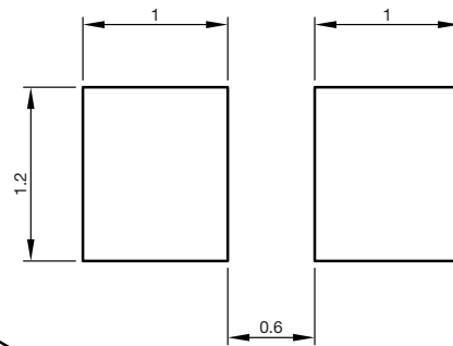
Recommended solder pad Footprint
