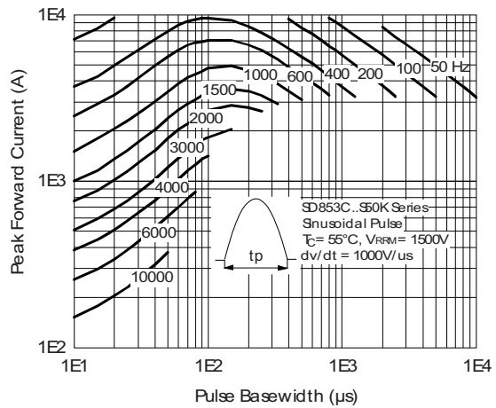
Fig. 16 - Frequency Characteristics
