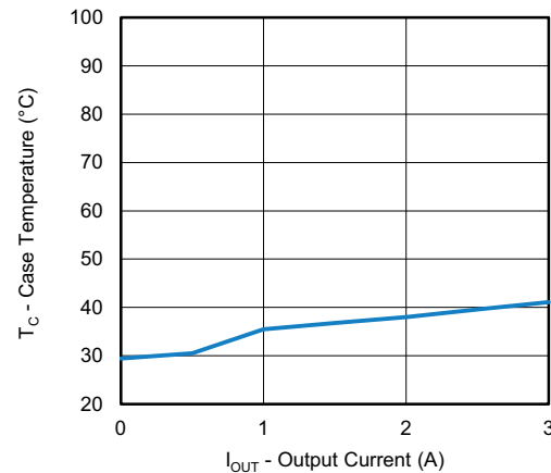
Fig. 33 - SiC479 Load Current vs. Case Temperature, VIN = 48 V, VOUT = 12 V
