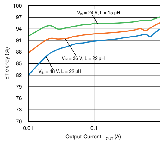
Fig. 32 - SiC479 Efficiency vs. Output Current - Light Load, VOUT = 12 V
