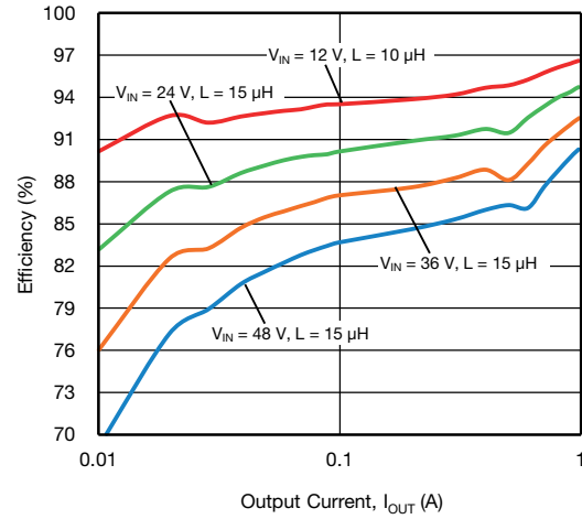
Fig. 31 - SiC479 Efficiency vs. Output Current - Light Load, VOUT = 5 V
