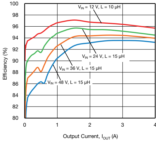
Fig. 28 - SiC479 Efficiency vs. Output Current, VOUT = 5 V
