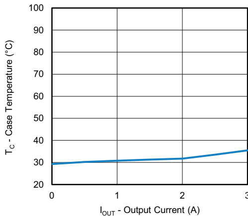
Fig. 30 - SiC479 Load Current vs. Case Temperature, VIN = 48 V, VOUT = 5 V
