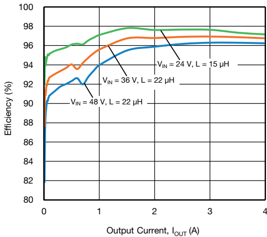
Fig. 29 - SiC479 Efficiency vs. Output Current, VOUT = 12 V
