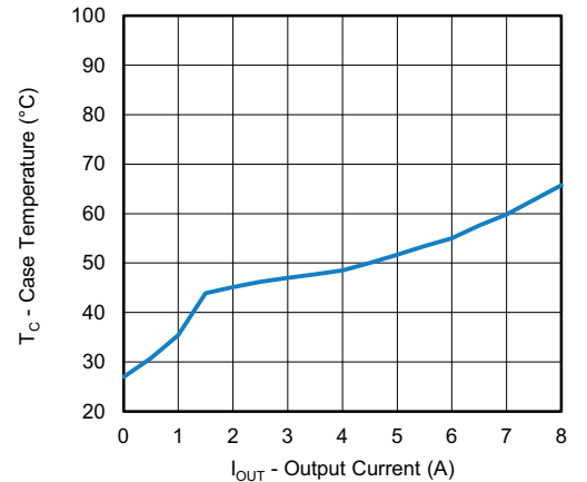
Fig. 21 - SiC477 Load Current vs. Case Temperature, V_{IN} = 48\text{ V}, V_{OUT} = 12\text{ V}
