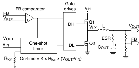
Fig. 24 - On-Time Generation
