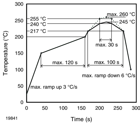
Fig. 9 - Lead (Pb)-free Reflow Solder Profile According to J-STD-020 for SMD Devices
