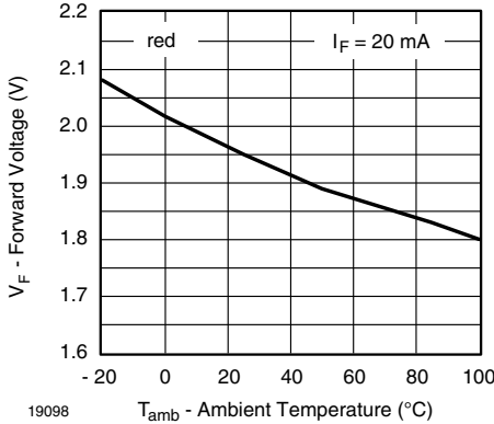
Fig. 8 - Forward Voltage vs. Ambient Temperature
