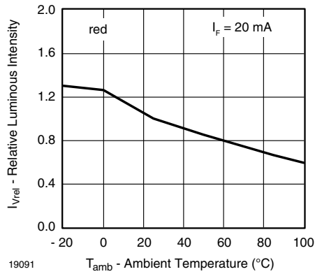
Fig. 7 - Relative Luminous Intensity vs. Ambient Temperature
