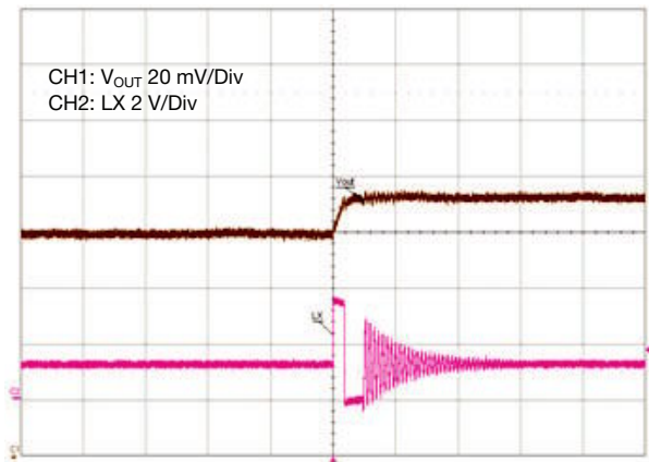
Output Ripple PSM: 0 A Load
