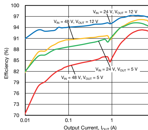
Fig. 2 - SiC472 Efficiency vs. Output Current
