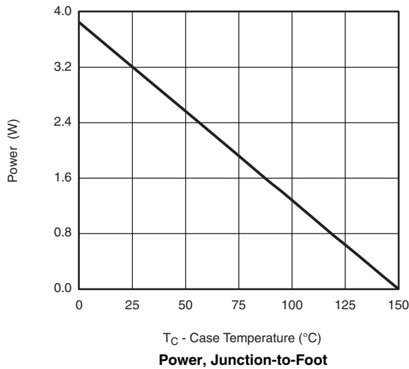
Power, Junction-to-Foot
